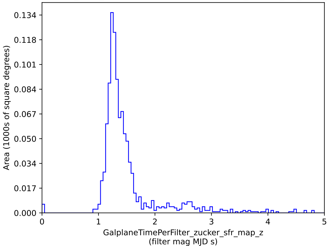
baseline_v2.1_10yrs : GalplaneTimePerFilter_zucker_sfr_map_z
