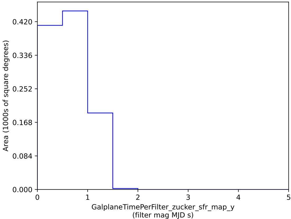
baseline_v2.1_10yrs : GalplaneTimePerFilter_zucker_sfr_map_y
