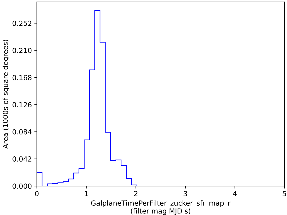
baseline_v2.1_10yrs : GalplaneTimePerFilter_zucker_sfr_map_r
