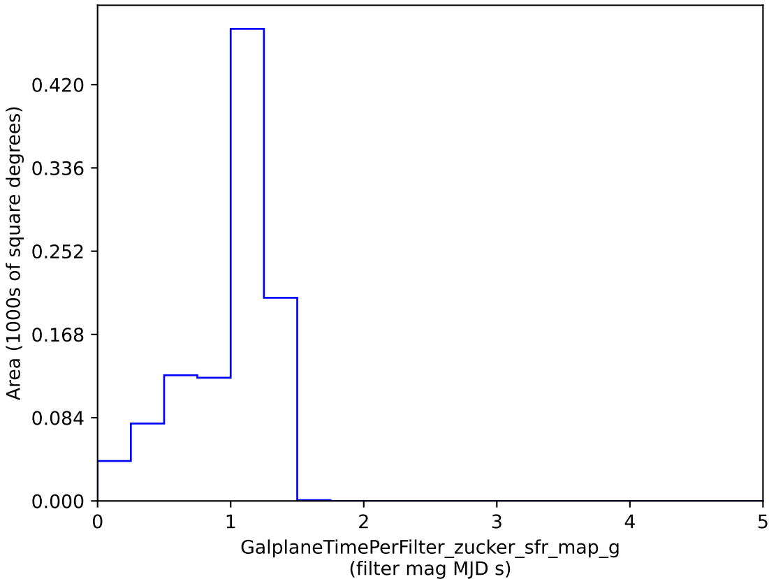
baseline_v2.1_10yrs : GalplaneTimePerFilter_zucker_sfr_map_g
