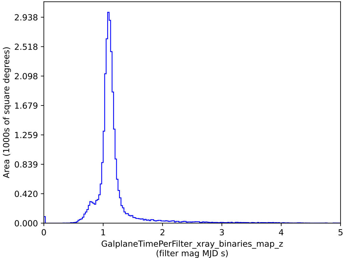
baseline_v2.1_10yrs : GalplaneTimePerFilter_xray_binaries_map_z
