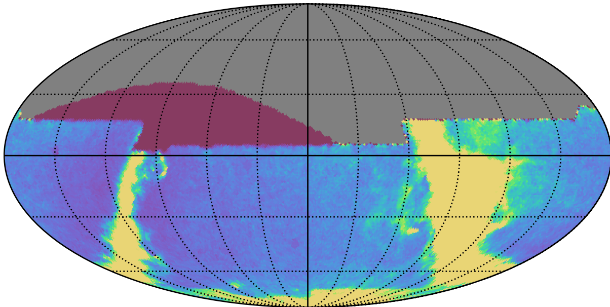
baseline_v2.1_10yrs : GalplaneTimePerFilter_xray_binaries_map_u
