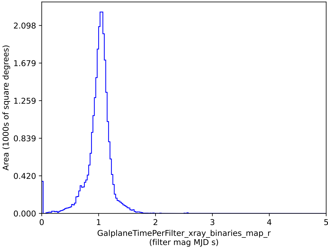
baseline_v2.1_10yrs : GalplaneTimePerFilter_xray_binaries_map_r
