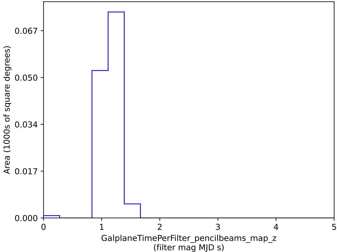
baseline_v2.1_10yrs : GalplaneTimePerFilter_pencilbeams_map_z
