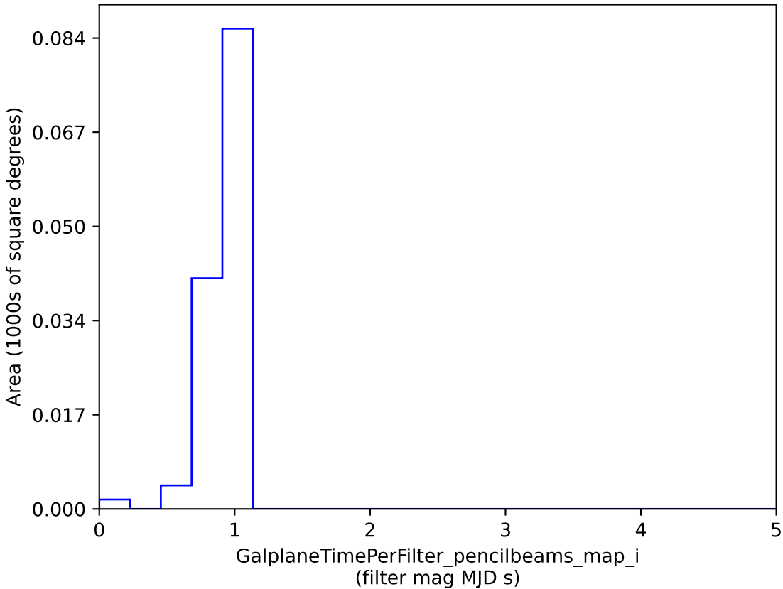
baseline_v2.1_10yrs : GalplaneTimePerFilter_pencilbeams_map_i
