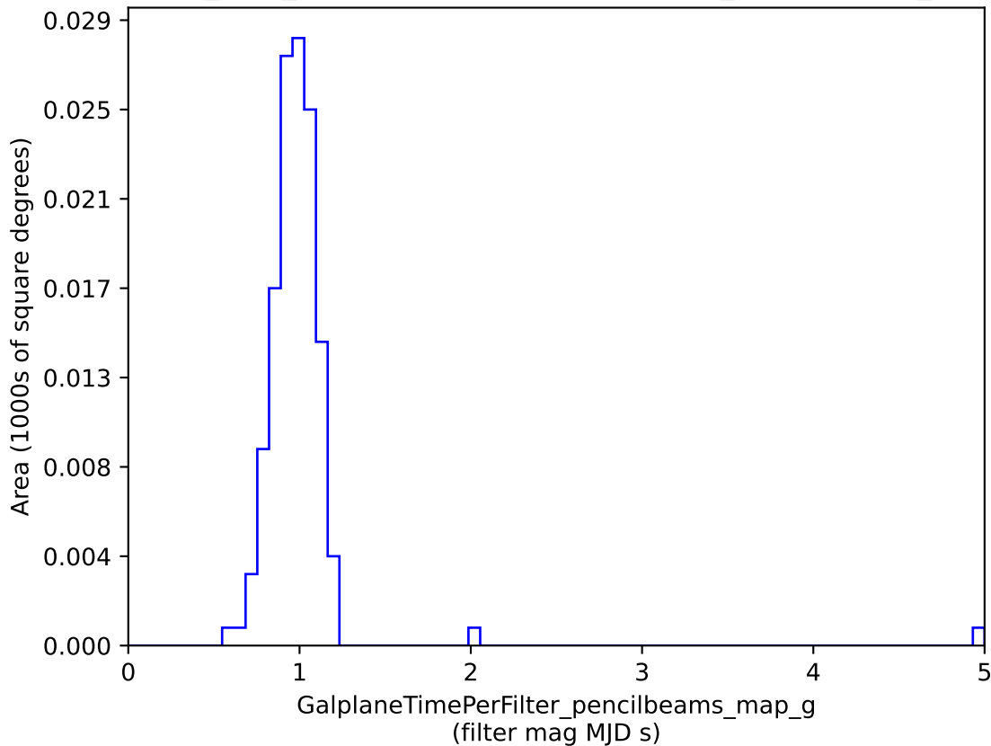
baseline_v2.1_10yrs : GalplaneTimePerFilter_pencilbeams_map_g
