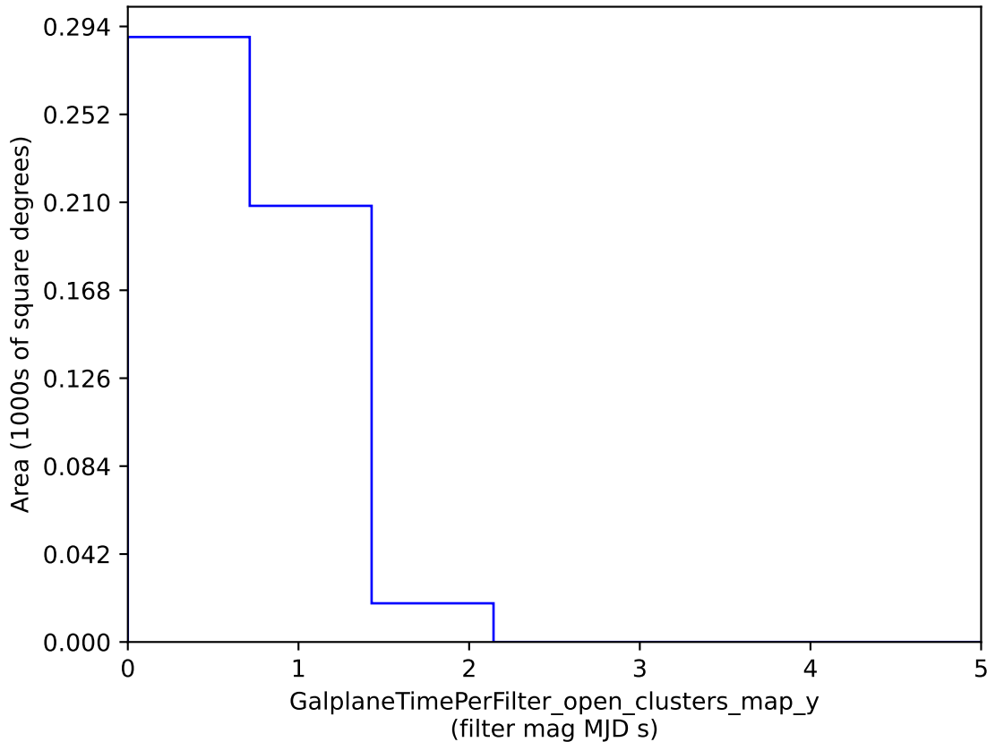
baseline_v2.1_10yrs : GalplaneTimePerFilter_open_clusters_map_y
