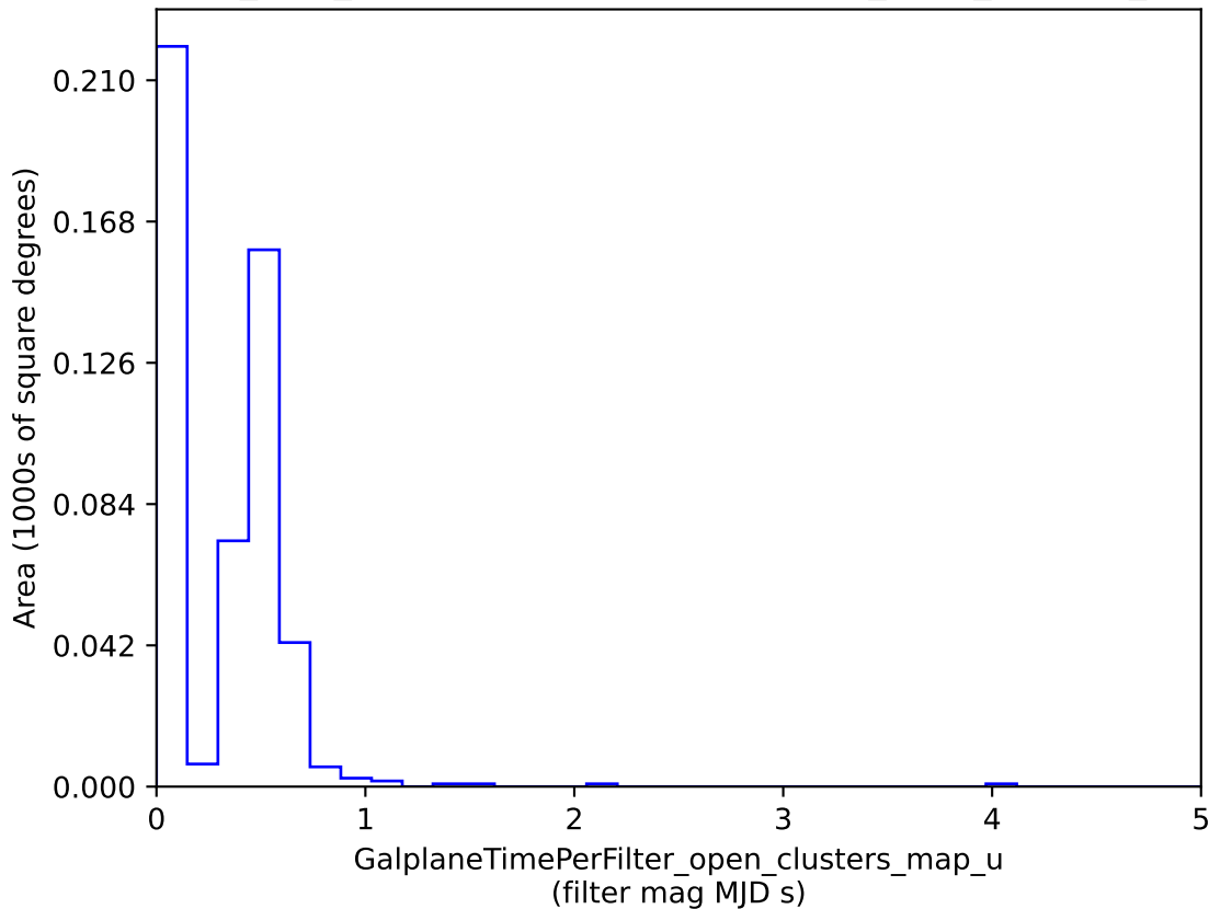
baseline_v2.1_10yrs : GalplaneTimePerFilter_open_clusters_map_u
