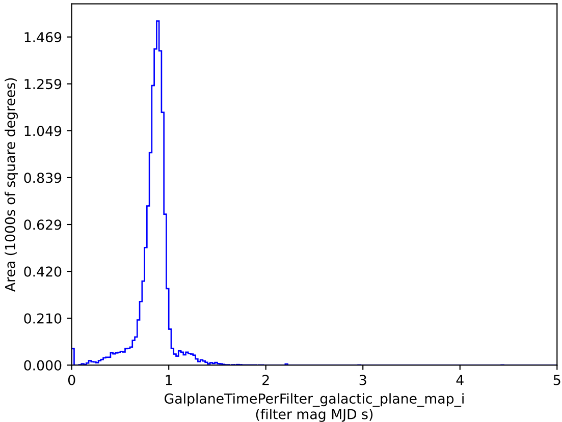
baseline_v2.1_10yrs : GalplaneTimePerFilter_galactic_plane_map_i
