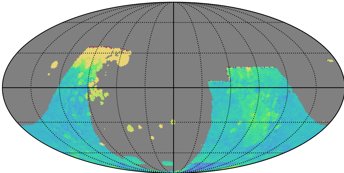
baseline_v2.1_10yrs : GalplaneTimePerFilter_combined_map_z
