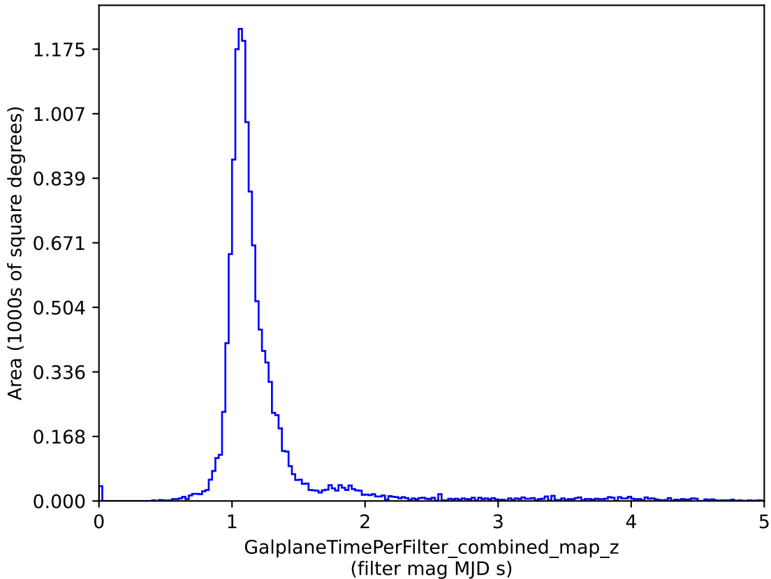
baseline_v2.1_10yrs : GalplaneTimePerFilter_combined_map_z
