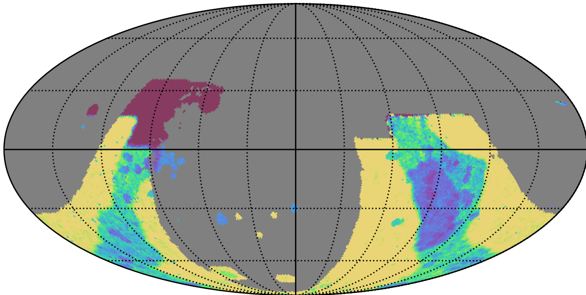
baseline_v2.1_10yrs : GalplaneTimePerFilter_combined_map_y
