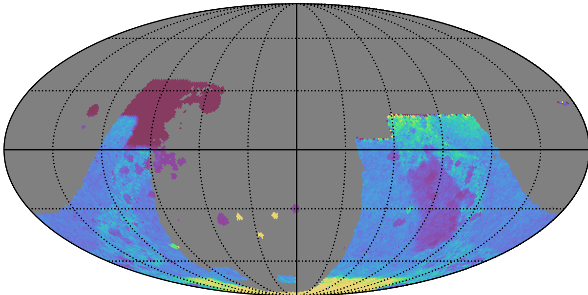
baseline_v2.1_10yrs : GalplaneTimePerFilter_combined_map_u
