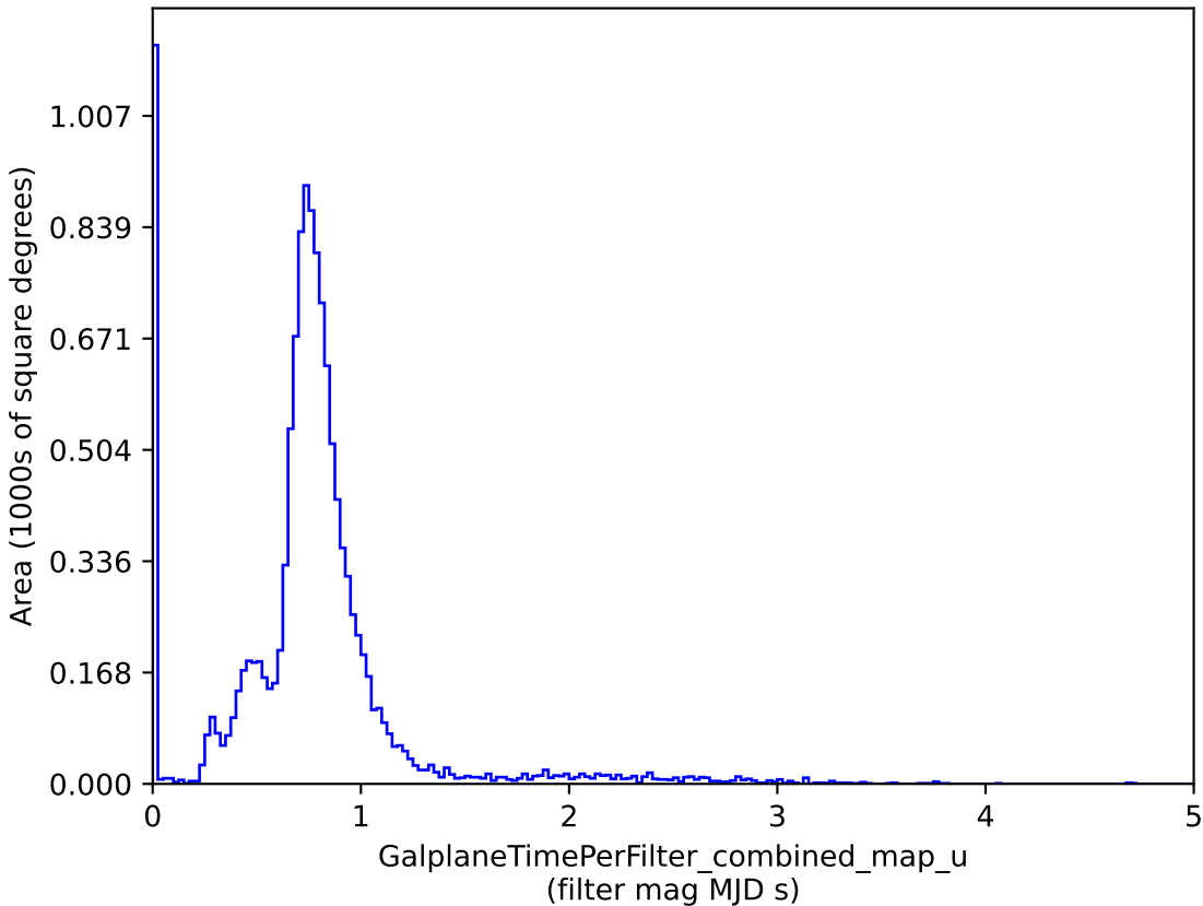
baseline_v2.1_10yrs : GalplaneTimePerFilter_combined_map_u
