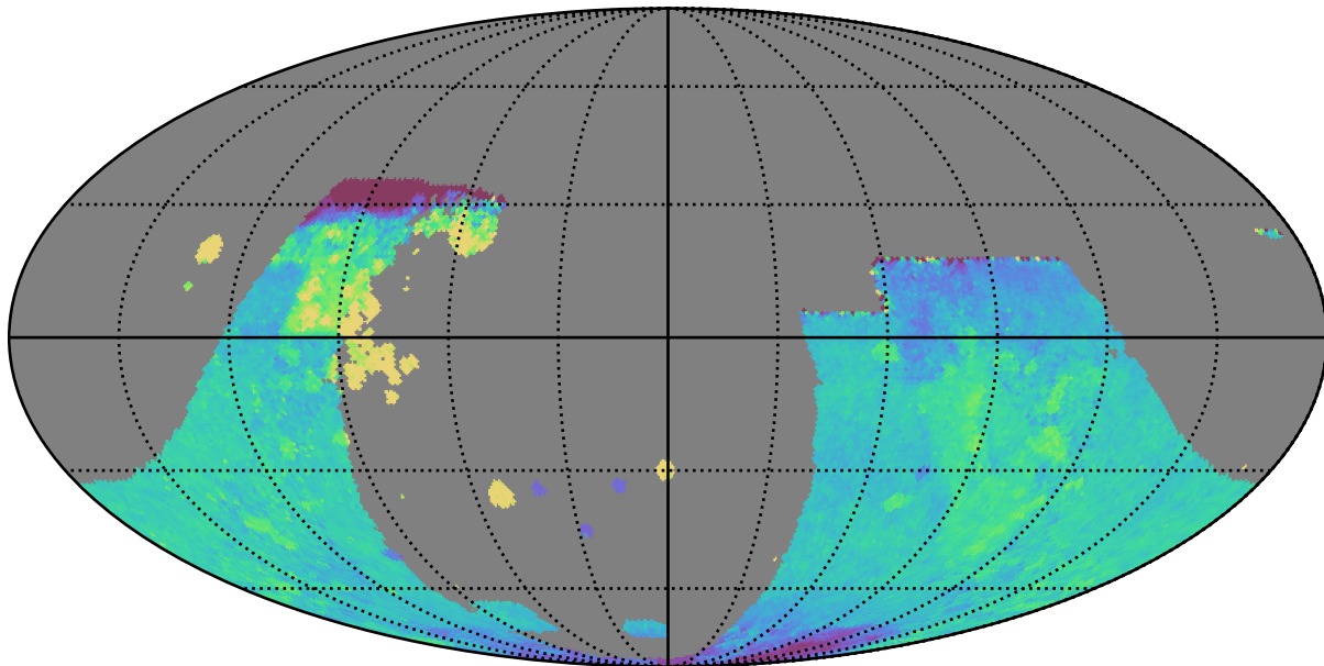
baseline_v2.1_10yrs : GalplaneTimePerFilter_combined_map_r
