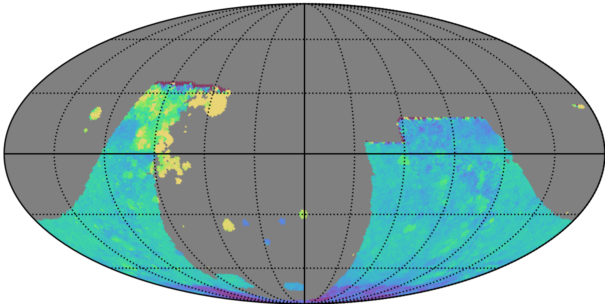
baseline_v2.1_10yrs : GalplaneTimePerFilter_combined_map_i
