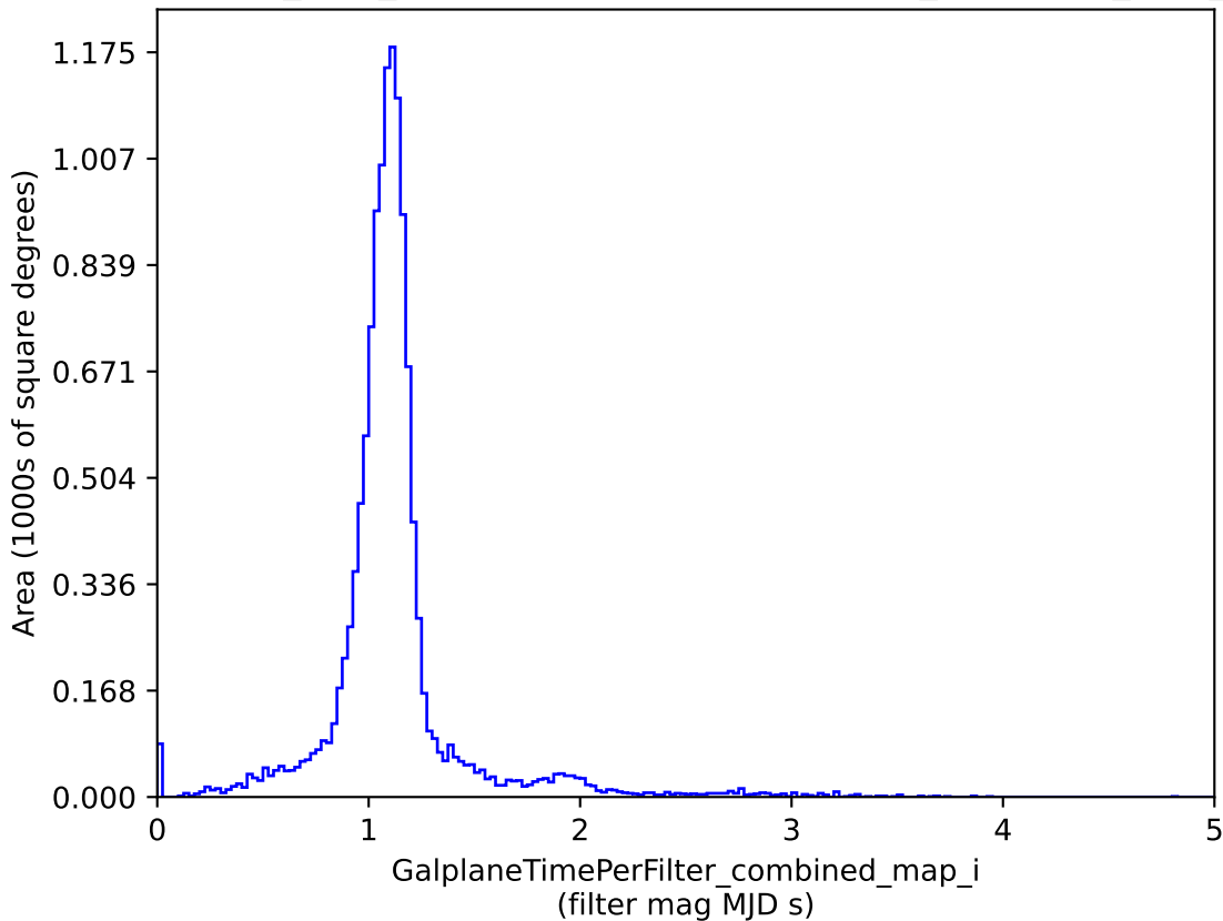
baseline_v2.1_10yrs : GalplaneTimePerFilter_combined_map_i
