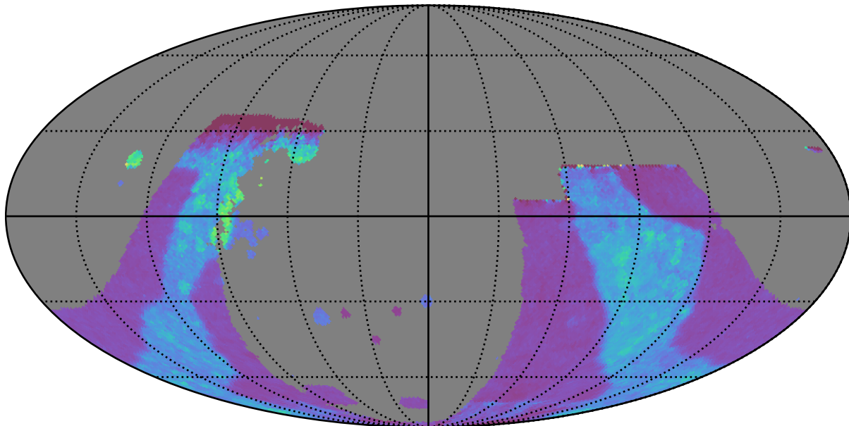
baseline_v2.1_10yrs : GalplaneTimePerFilter_combined_map_g
