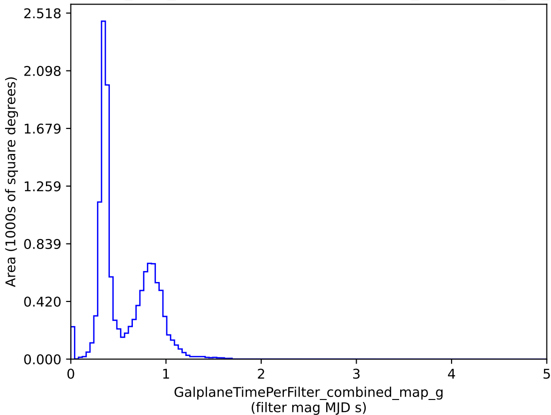
baseline_v2.1_10yrs : GalplaneTimePerFilter_combined_map_g
