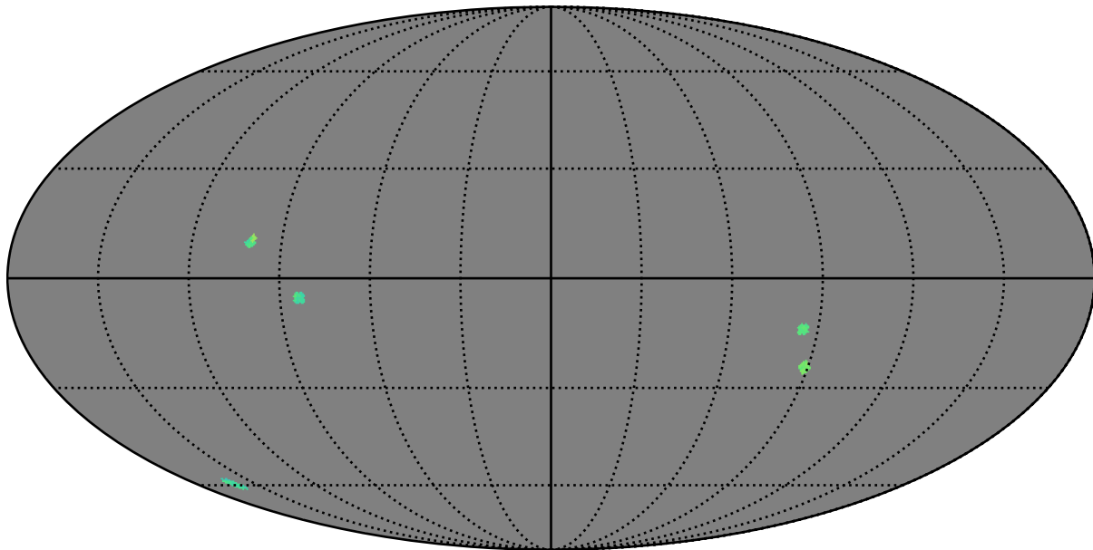
baseline_v2.1_10yrs : GalplaneTimePerFilter_bonito_sfr_map_z
