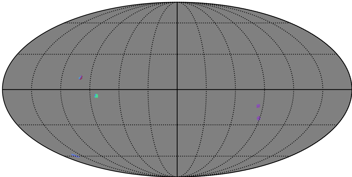
baseline_v2.1_10yrs : GalplaneTimePerFilter_bonito_sfr_map_y
