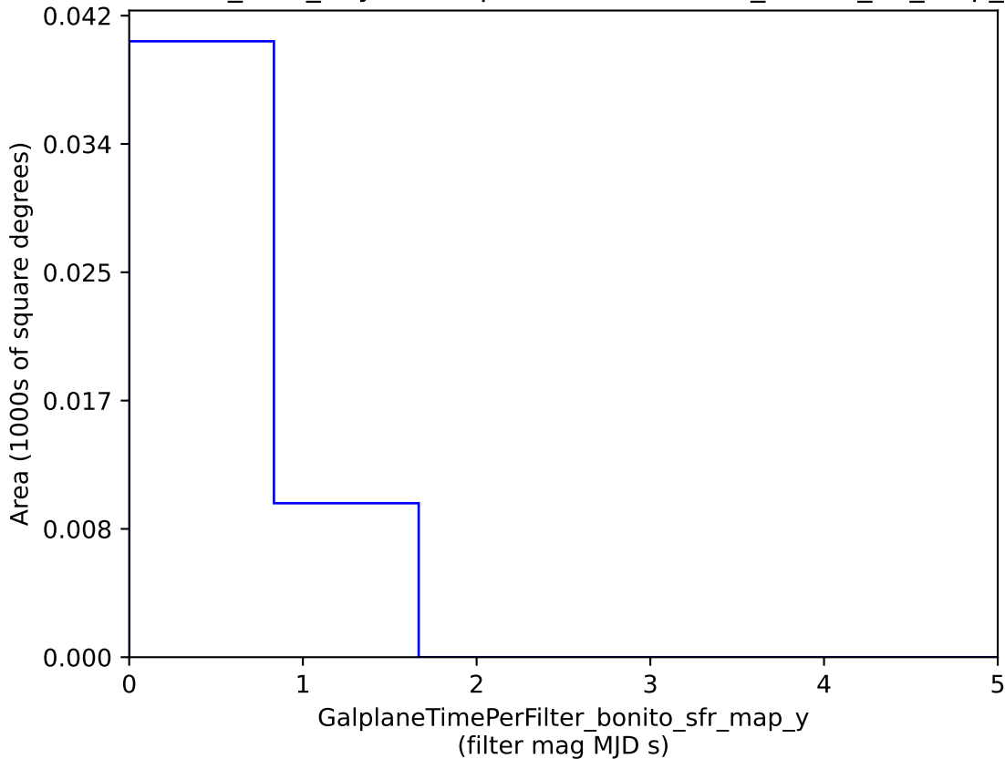
baseline_v2.1_10yrs : GalplaneTimePerFilter_bonito_sfr_map_y
