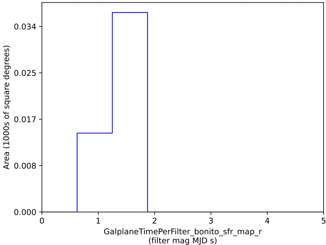
baseline_v2.1_10yrs : GalplaneTimePerFilter_bonito_sfr_map_r
