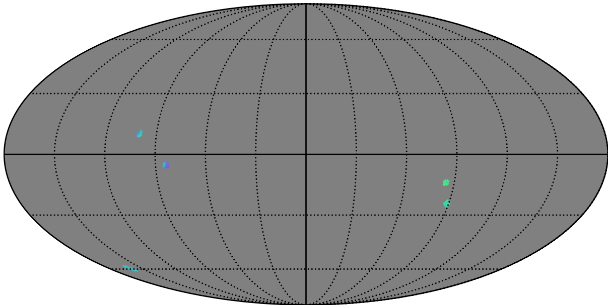
baseline_v2.1_10yrs : GalplaneTimePerFilter_bonito_sfr_map_g
