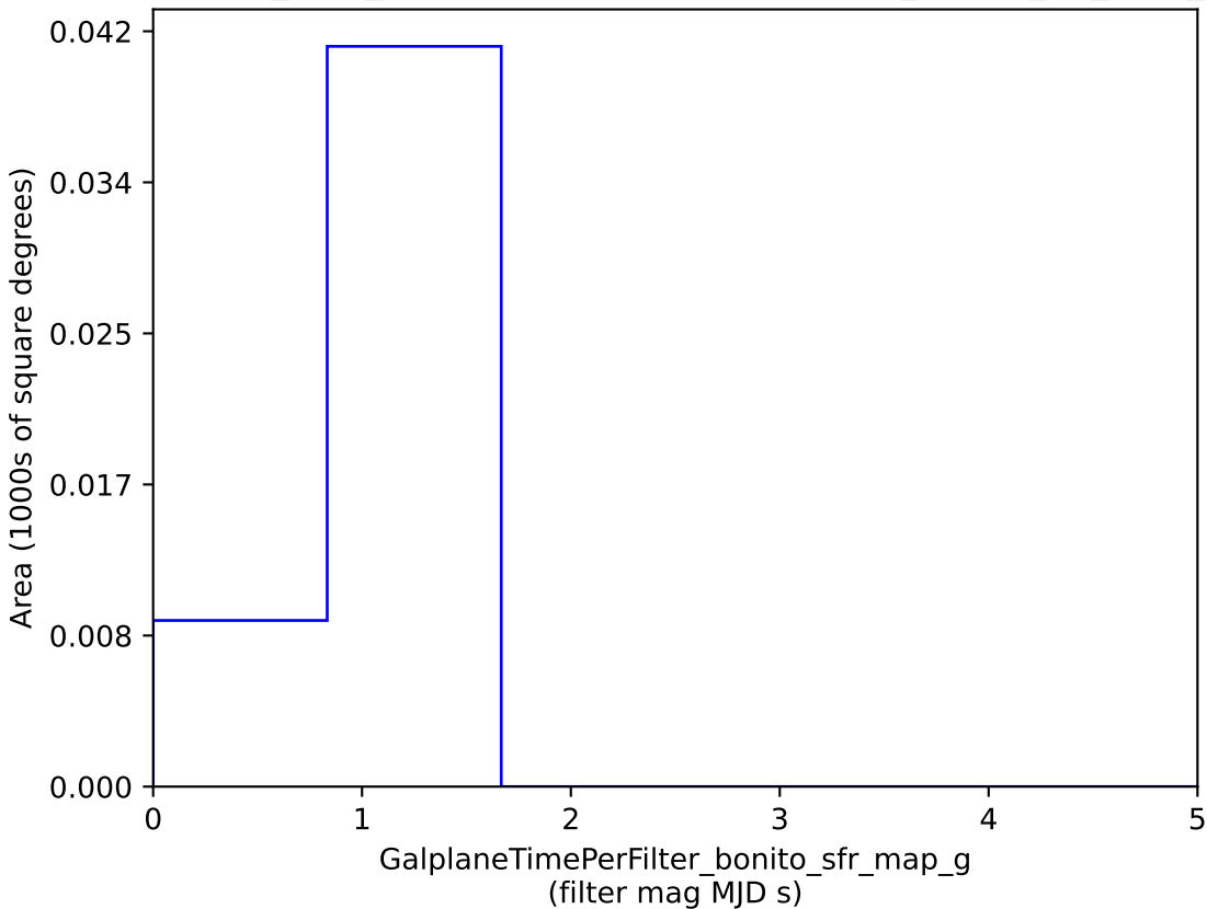
baseline_v2.1_10yrs : GalplaneTimePerFilter_bonito_sfr_map_g
