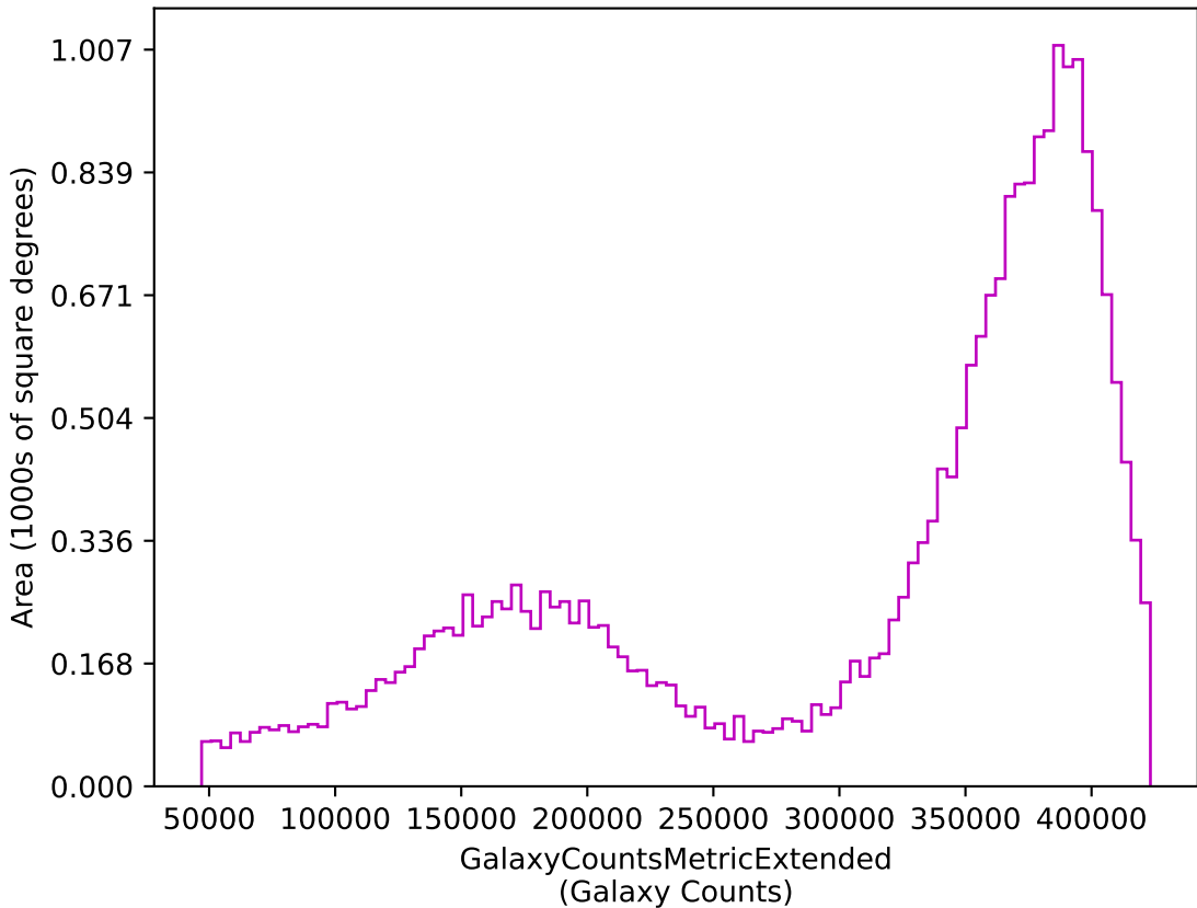
baseline_v2.1_10yrs z: GalaxyCountsMetricExtended
