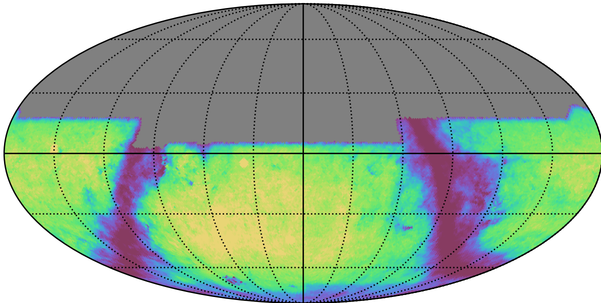
baseline_v2.1_10yrs u: GalaxyCountsMetricExtended
