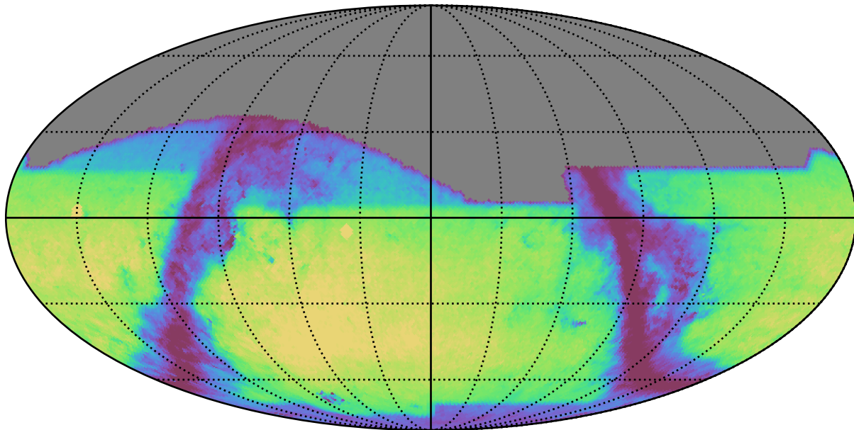
baseline_v2.1_10yrs r: GalaxyCountsMetricExtended
