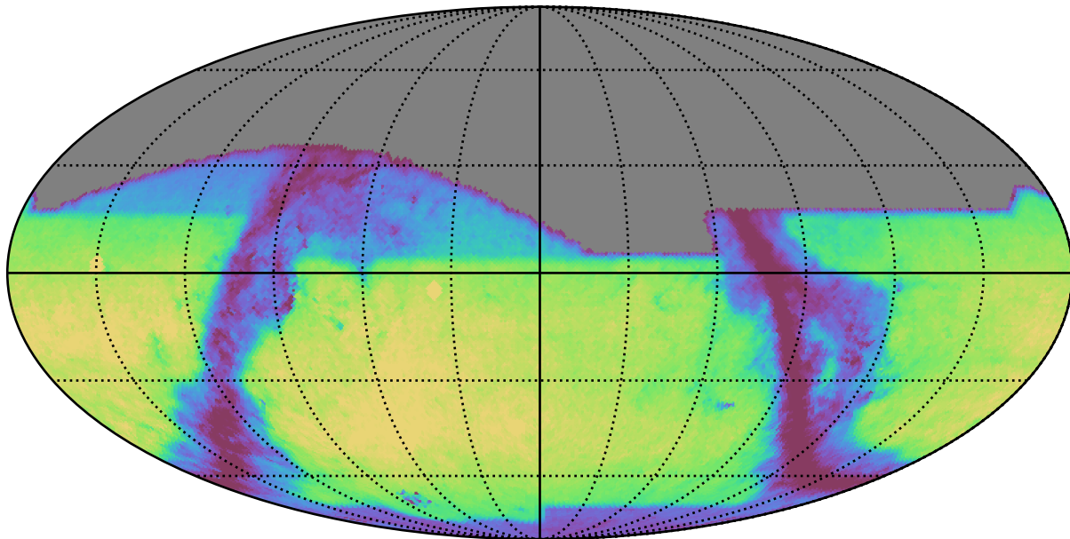
baseline_v2.1_10yrs i: GalaxyCountsMetricExtended
