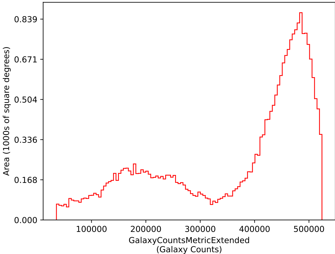
baseline_v2.1_10yrs i: GalaxyCountsMetricExtended
