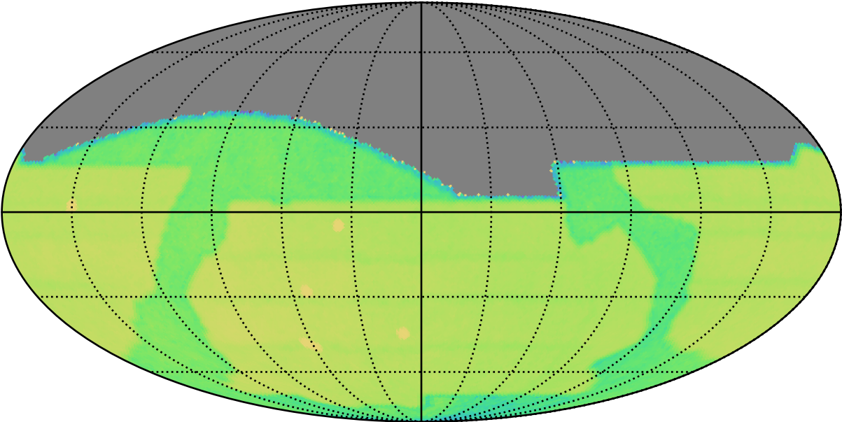
baseline_v2.1_10yrs : GalPlaneVisitIntervalsTimescales_xray_binaries_map_Tau_5_0
