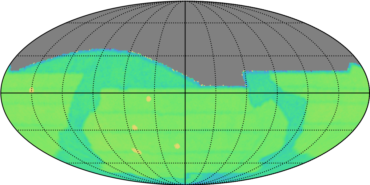
baseline_v2.1_10yrs : GalPlaneVisitIntervalsTimescales_xray_binaries_map_Tau_2_0
