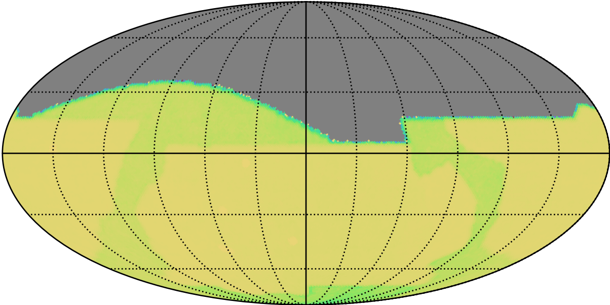
baseline_v2.1_10yrs : GalPlaneVisitIntervalsTimescales_xray_binaries_map_Tau_20_0
