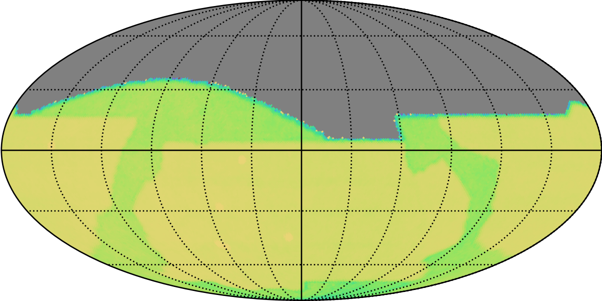
baseline_v2.1_10yrs : GalPlaneVisitIntervalsTimescales_xray_binaries_map_Tau_11_0
