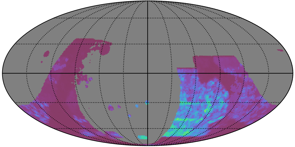
baseline_v2.1_10yrs : GalPlaneSeasonGapsTimescales_combined_map_Tau_55_0
