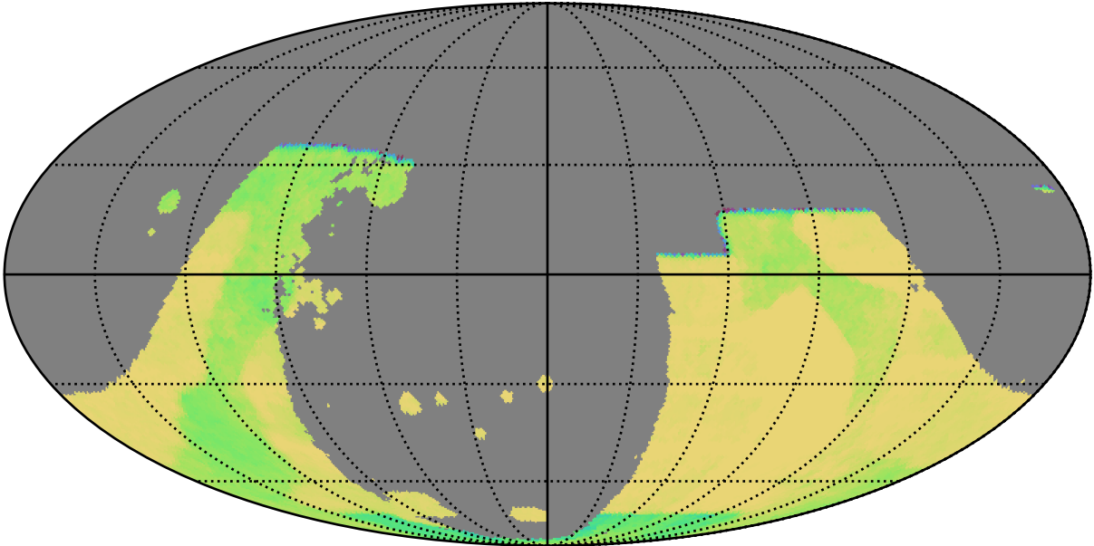
baseline_v2.1_10yrs : GalPlaneSeasonGapsTimescales_combined_map_Tau_232_5
