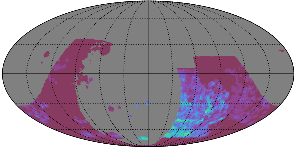
baseline_v2.1_10yrs : GalPlaneSeasonGapsTimescales_combined_map_Tau_10_0
