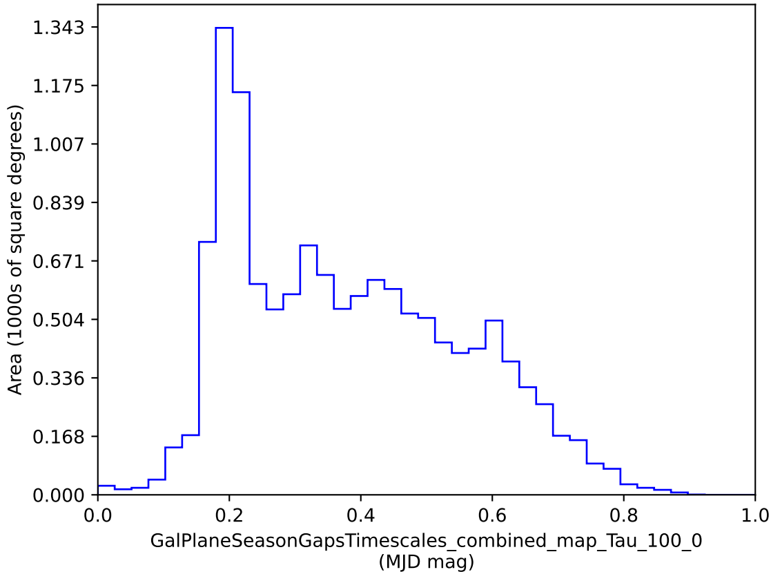
baseline_v2.1_10yrs : GalPlaneSeasonGapsTimescales_combined_map_Tau_100_0
