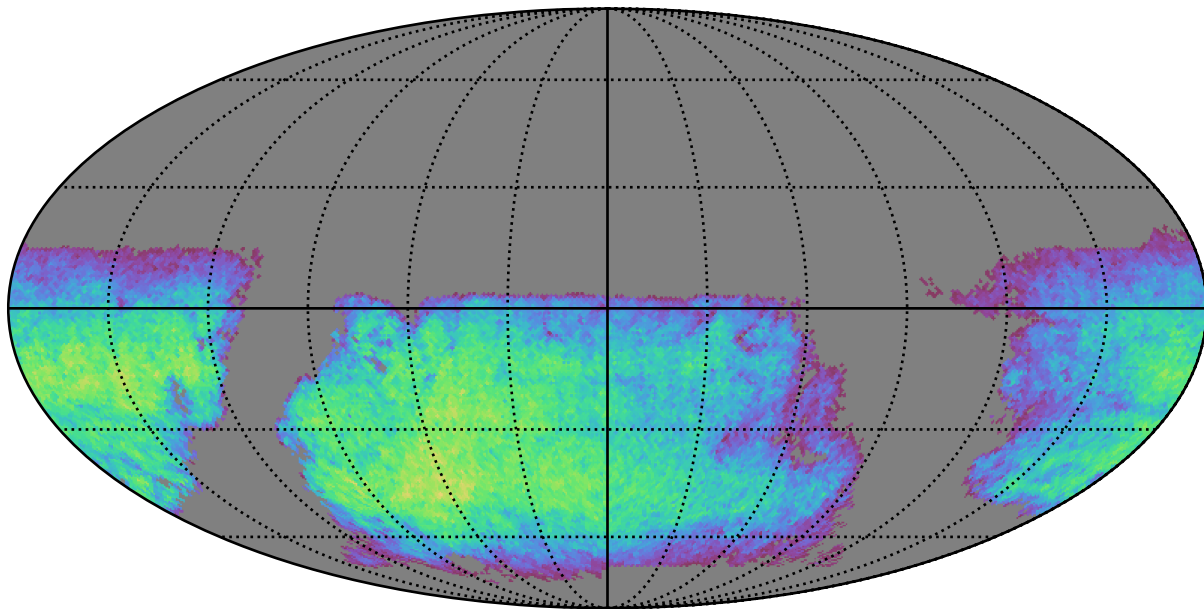
baseline_v2.1_10yrs i band non-DD year 9: ExgalM5WithCuts
