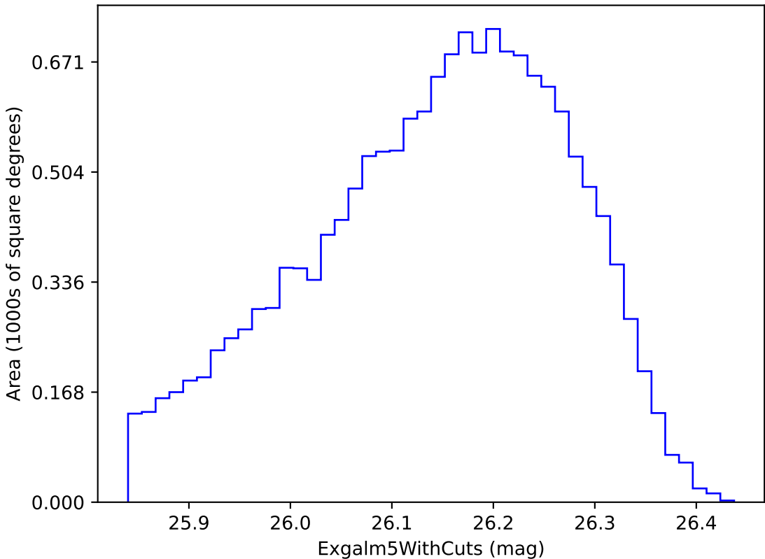
baseline_v2.1_10yrs i band non-DD year 9: ExgalM5WithCuts
