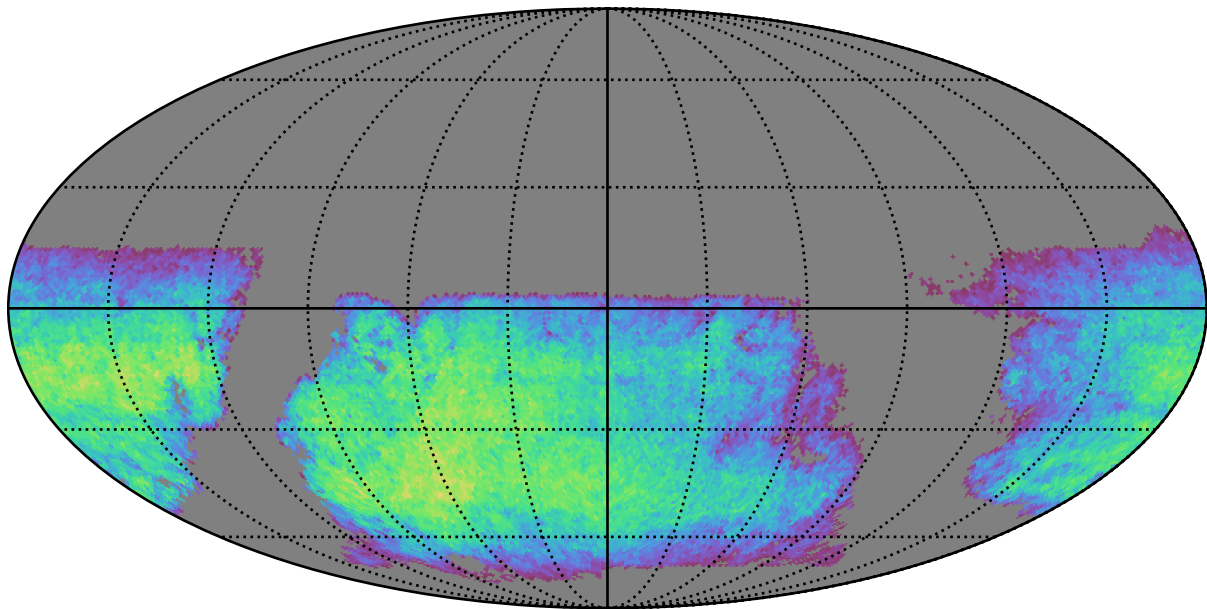
baseline_v2.1_10yrs i band non-DD year 8: ExgalM5WithCuts
