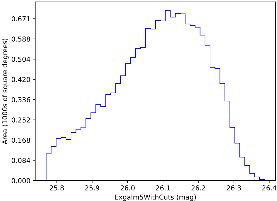
baseline_v2.1_10yrs i band non-DD year 8: ExgalM5WithCuts
