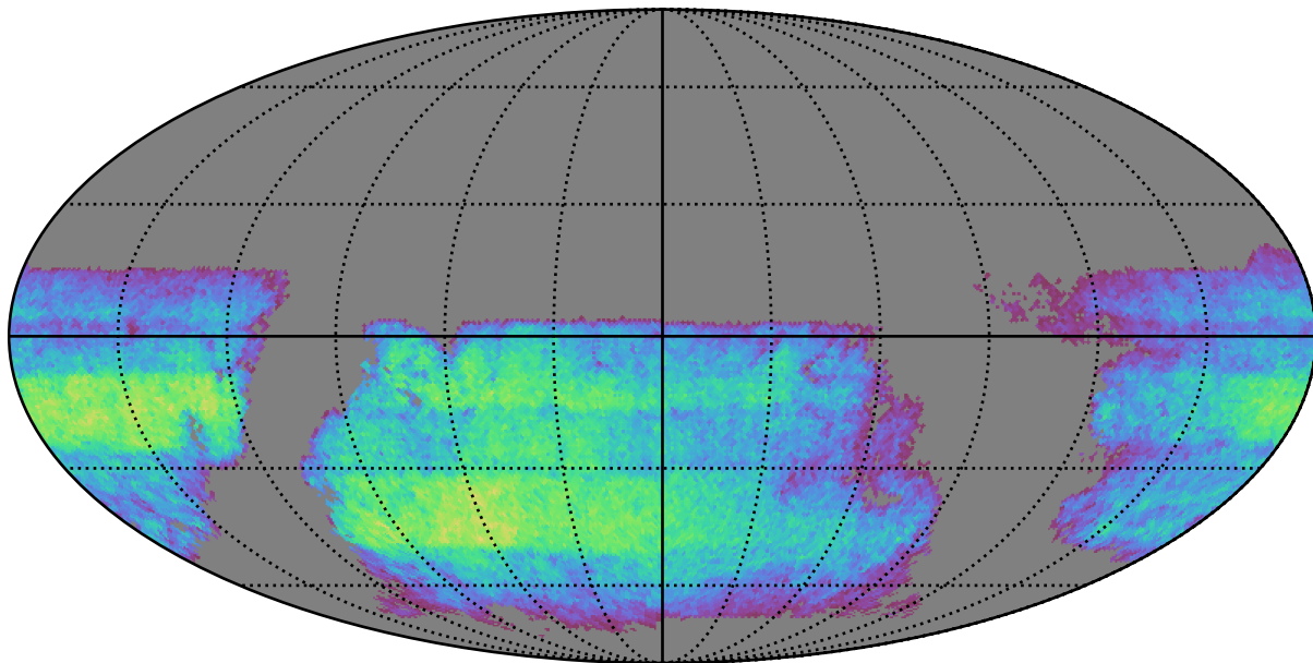
baseline_v2.1_10yrs i band non-DD year 7: ExgalM5WithCuts
