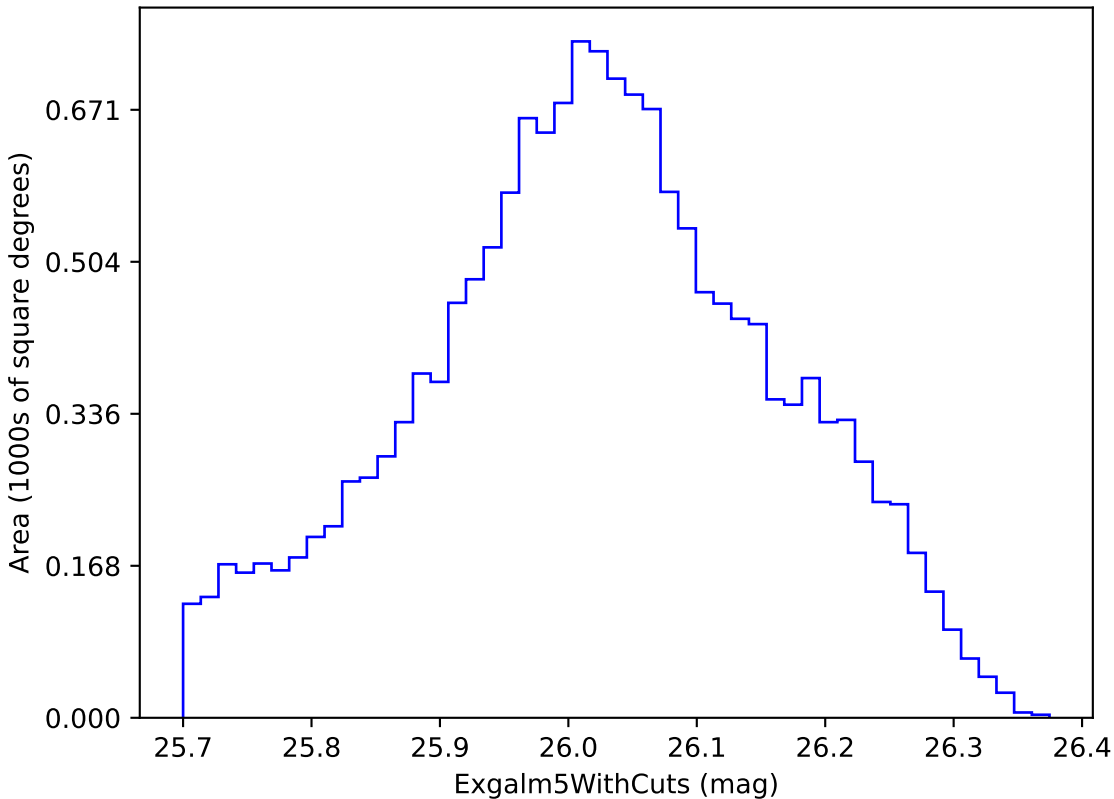
baseline_v2.1_10yrs i band non-DD year 7: ExgalM5WithCuts
