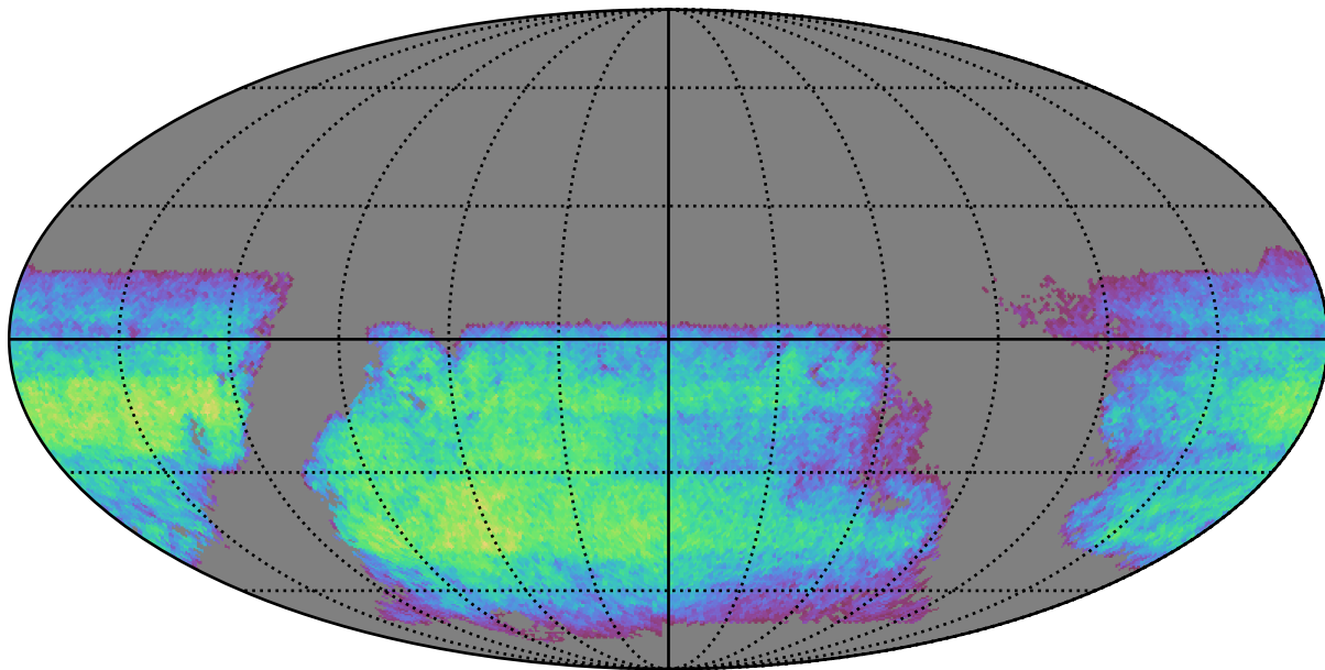
baseline_v2.1_10yrs i band non-DD year 6: ExgalM5WithCuts
