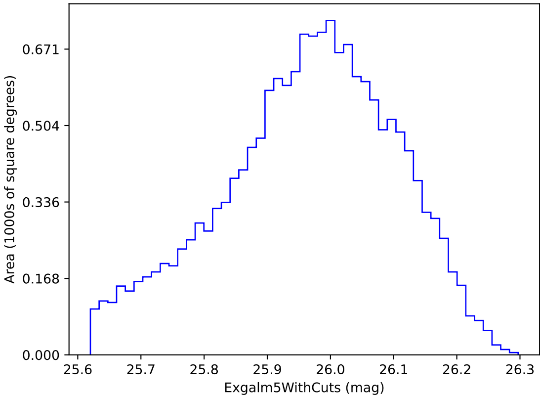
baseline_v2.1_10yrs i band non-DD year 6: ExgalM5WithCuts
